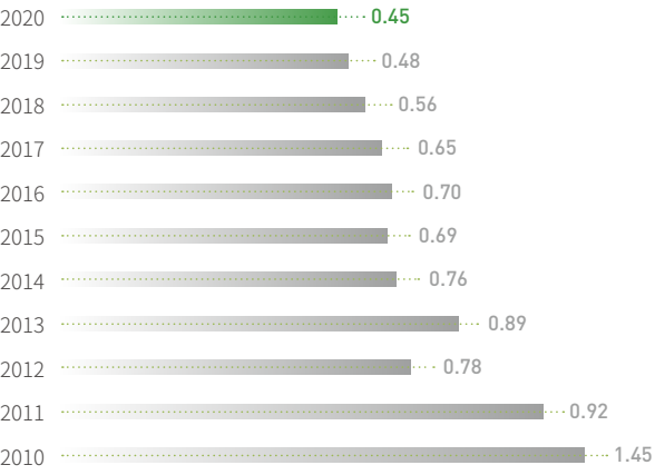
Nitrogen Oxide Emissions per Ton of Cement Clinker from 2010 to 2020 Unit: kg/ton
